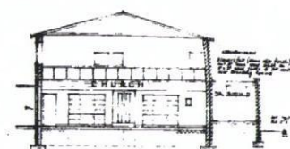
SECTION E-E
