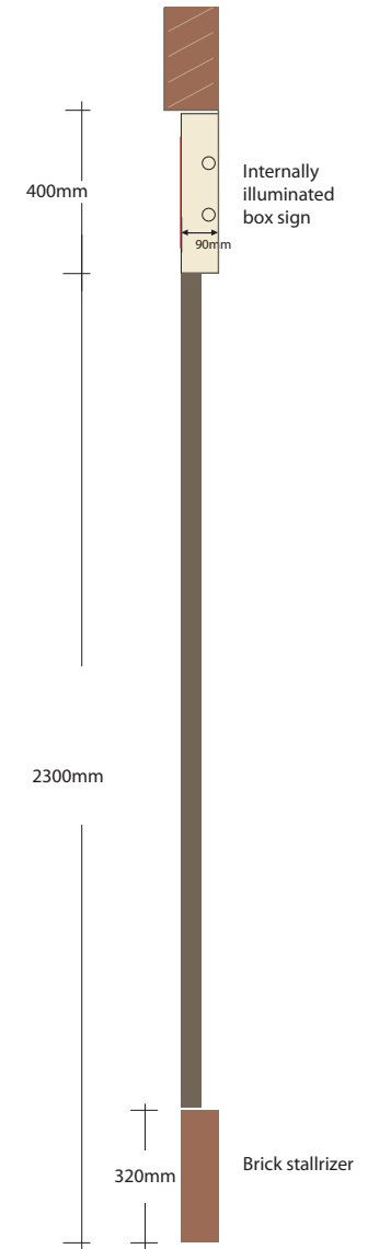
Section View
