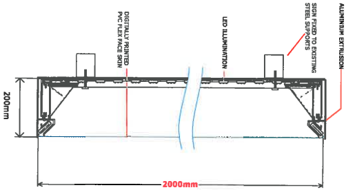
FLEXFACE SECTION THROUGH 1:20
