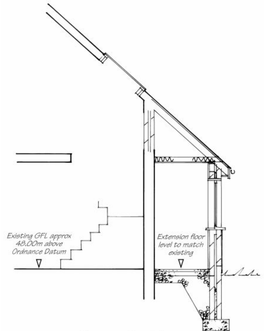
Cross-Section
