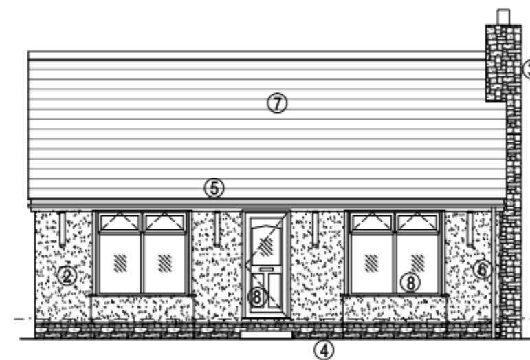
East Elevation
