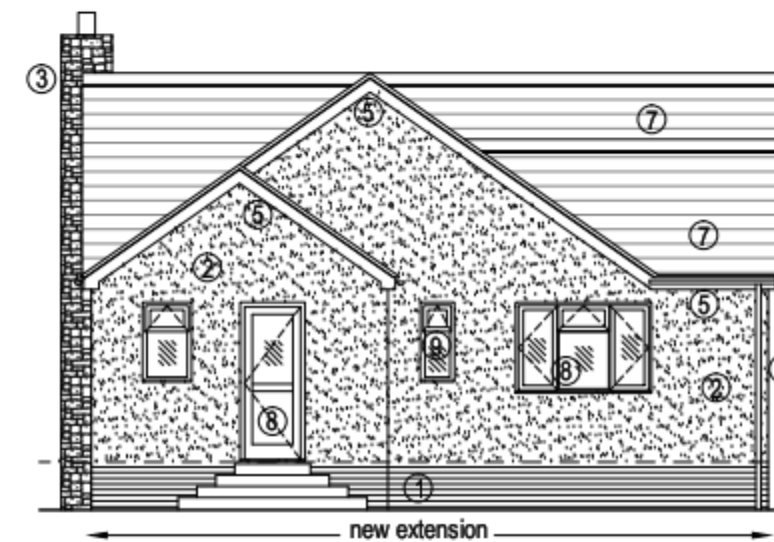
West Elevation
