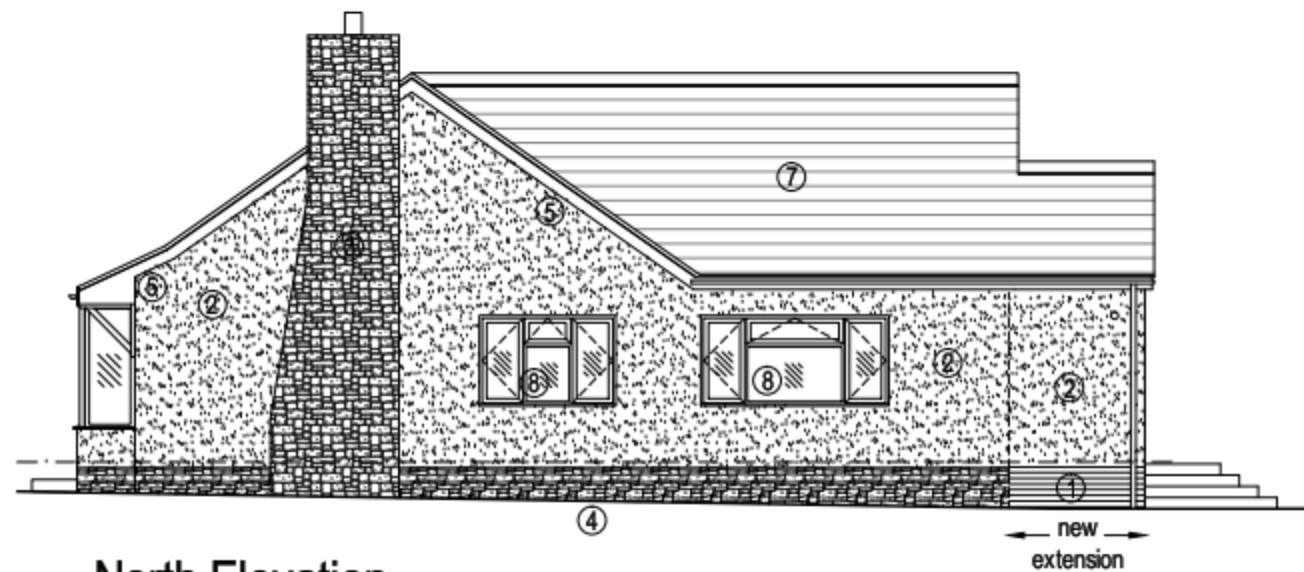
North Elevation
