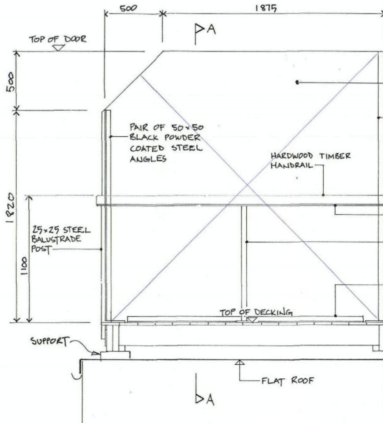
ELEVATION ON SCREEN 1:20
