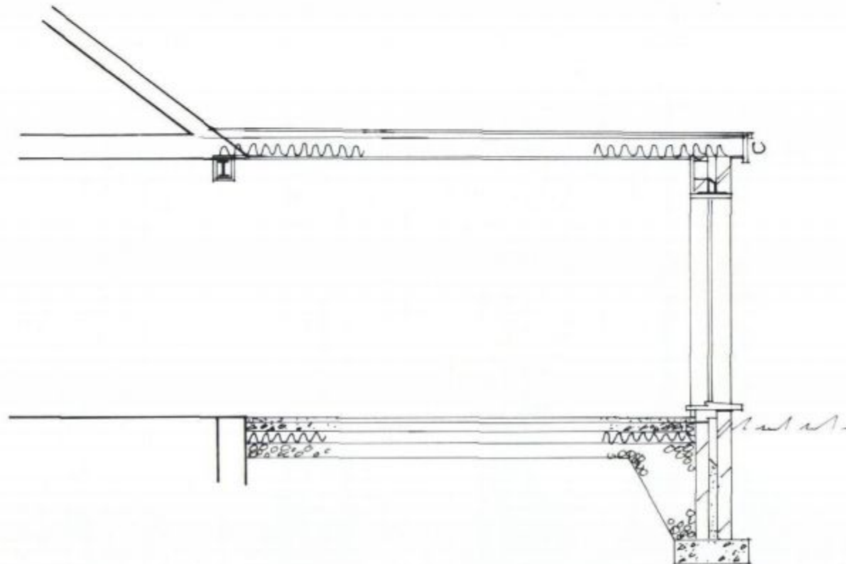
Cross-Section
