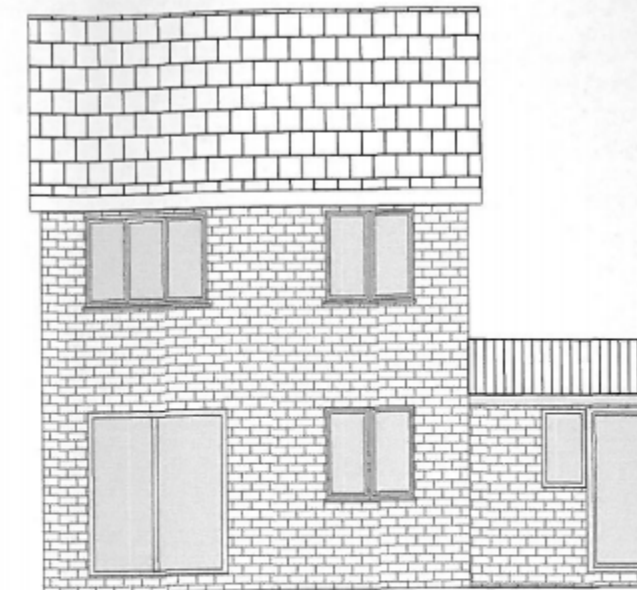
Existing East elevation Scale 1 : 100
