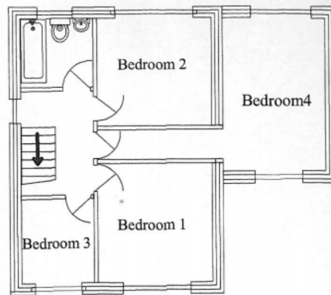
Proposed first floor Scale 1 : 100
