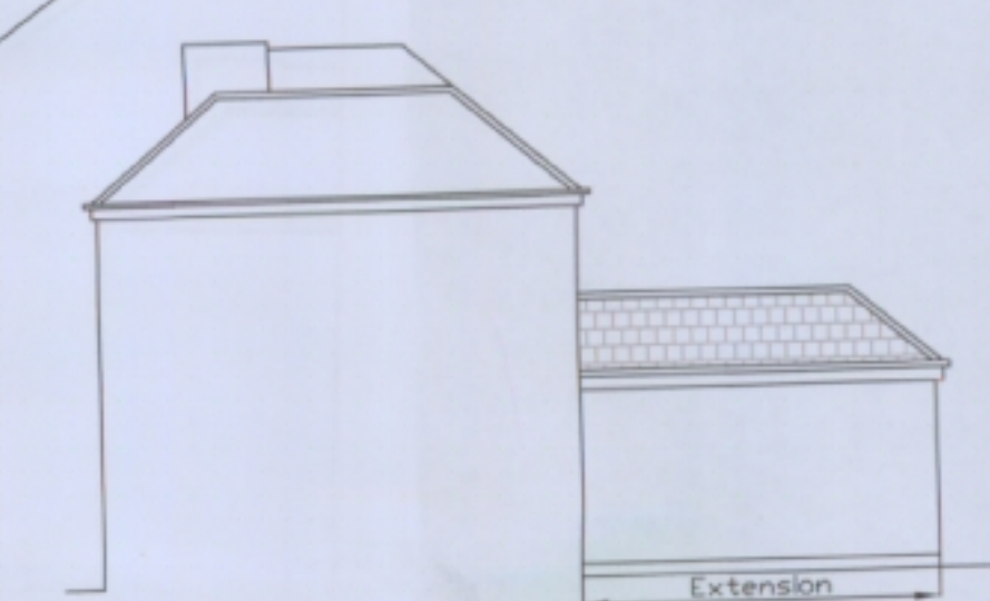
PROPOSED NORTH WEST ELEVATION
