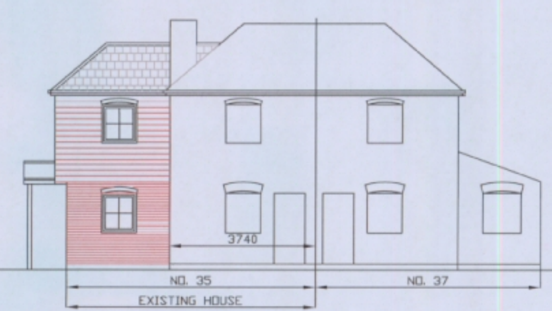
PROPOSED NORTH EAST (FRONT) ELEVATION
