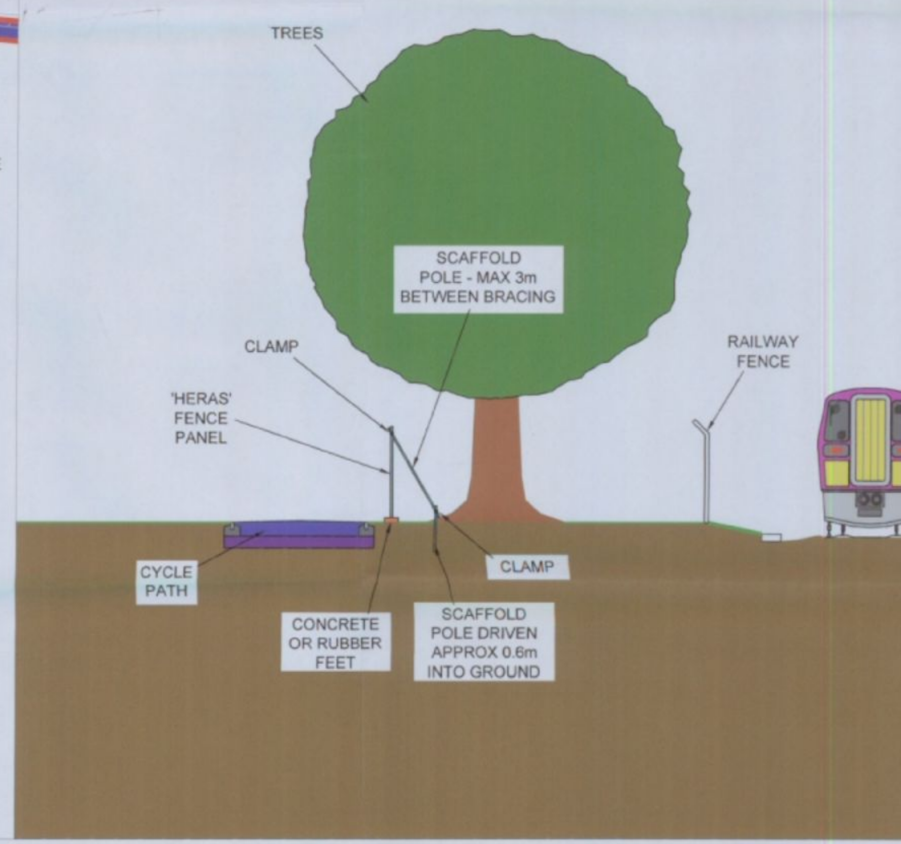
DETAIL OF TEMPORARY FENCING AROUND TREE DURING PATH CONSTRUCTION NOT TO SCALE
