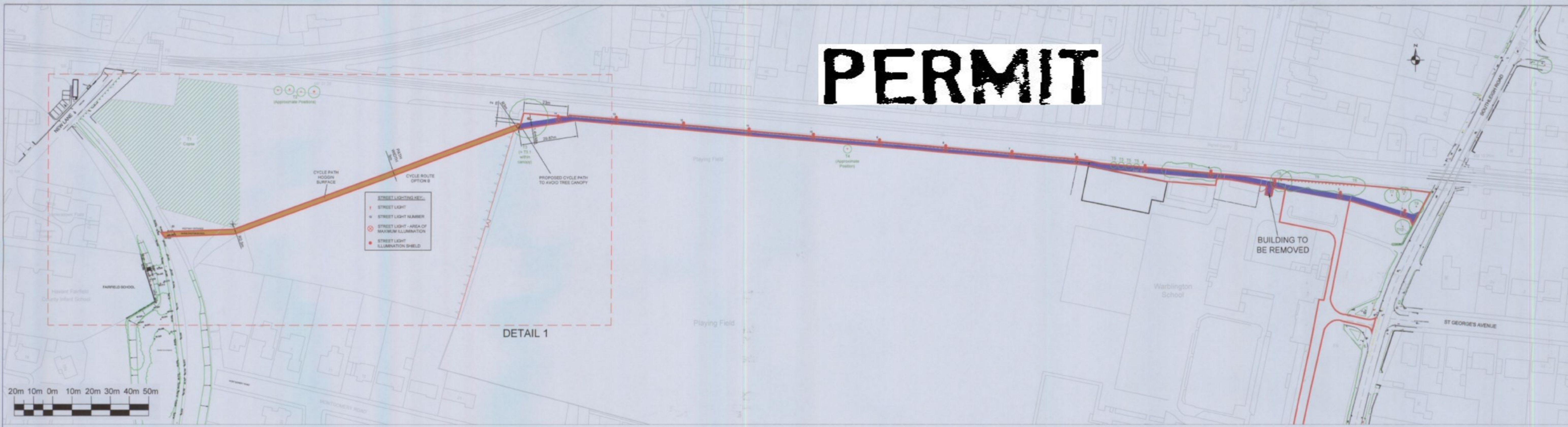
CYCLE PATH LOCATION PLAN SCALE 1:1000
