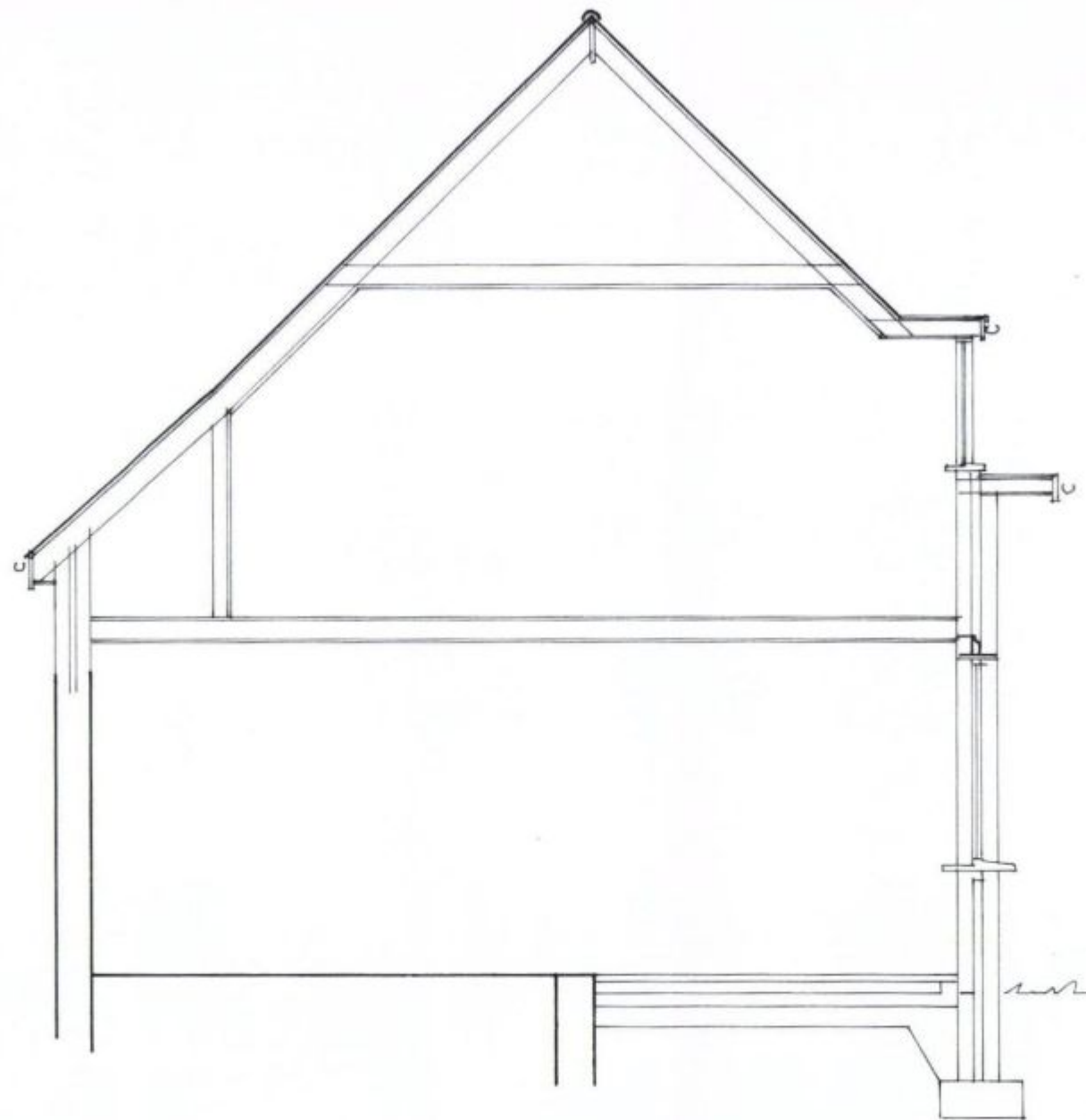
Cross-Section
