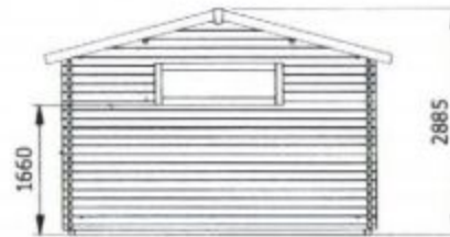
Elevation C
