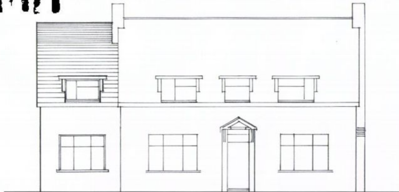
Proposed SW Elevation
