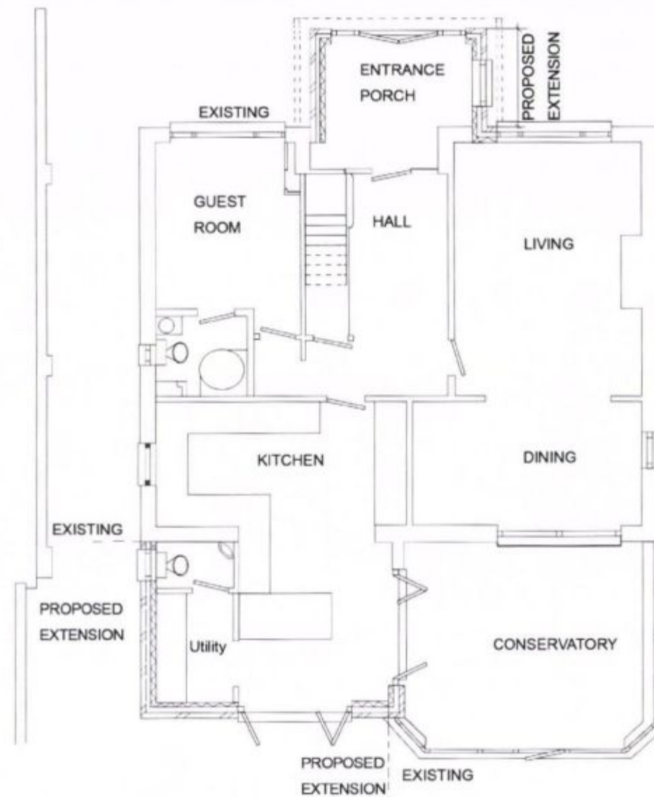
PROPOSED GROUND FLOOR PLAN DWG.NO: APP01-1
