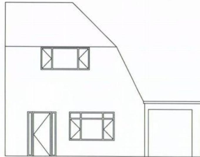
EXISTING SOUTH ELEVATION
