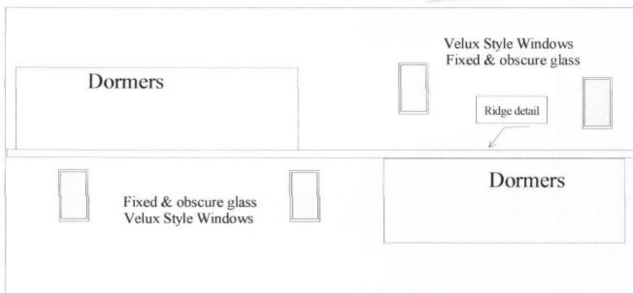
Proposed roof plan West elevation
