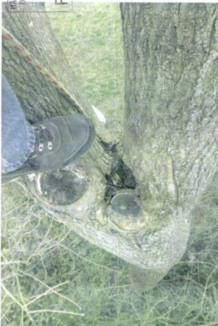
Photo 1 - defective attachment
