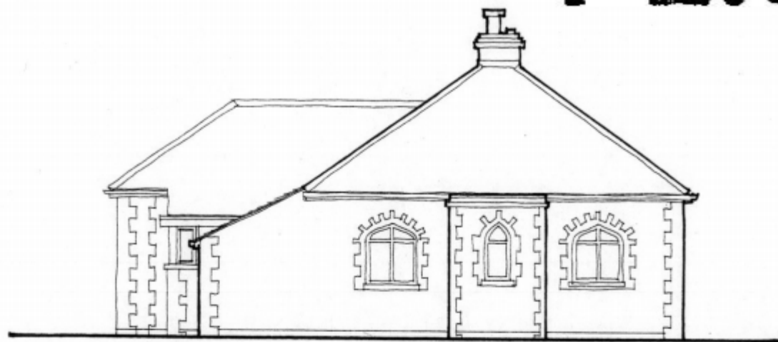
South Elevation (Ferry Road)
