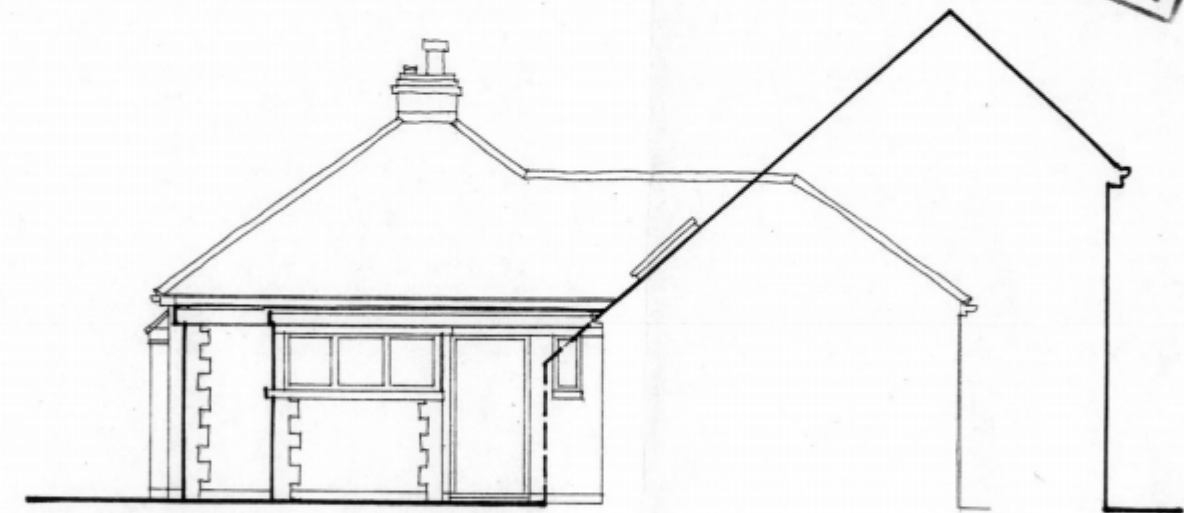
North Elevation
