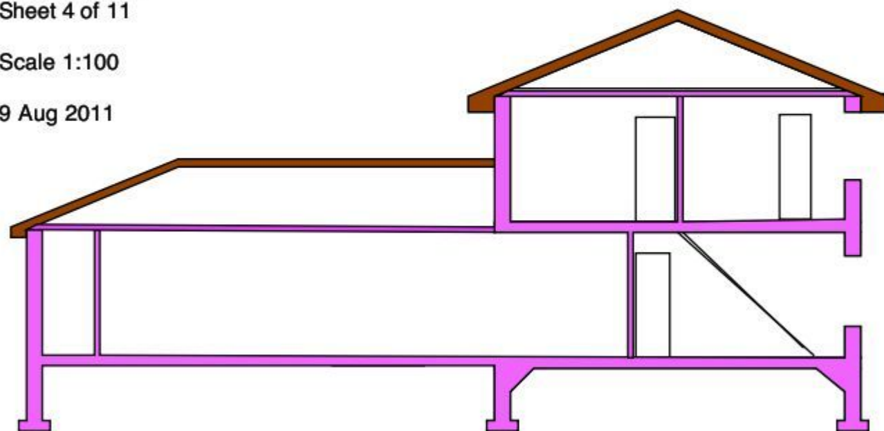
New Section Rear Single Storey Extension
