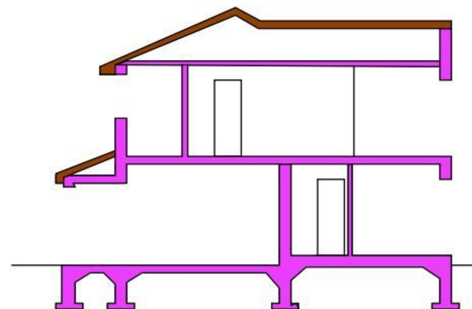
New Section Garage and Double Storey Extension
