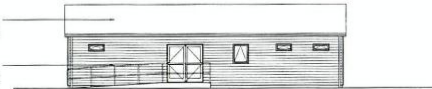
PROPOSED WEST ELEVATION 1:100
