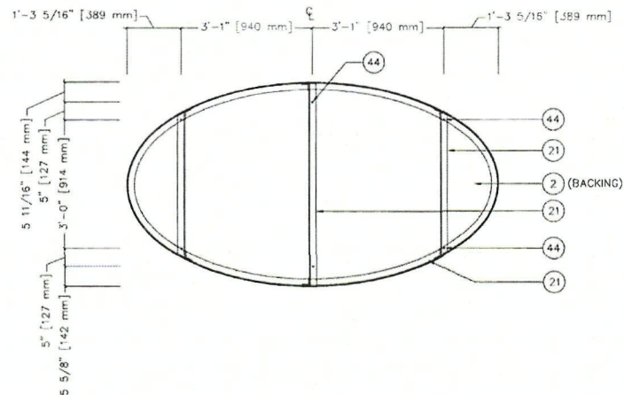
FRAMING/MOUNTING (ROTATED 11° FOR CLARITY)
