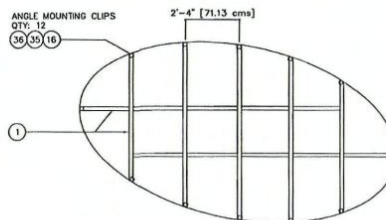
MOUNTING STRAPS DETAIL SCALE: 1/4"=1'-0"
