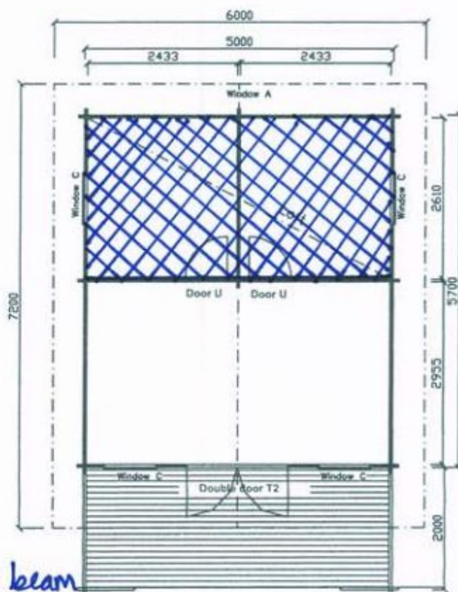
Ground plan
