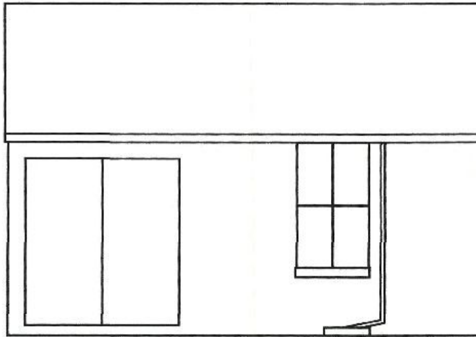
Small Store: South East Elevation
