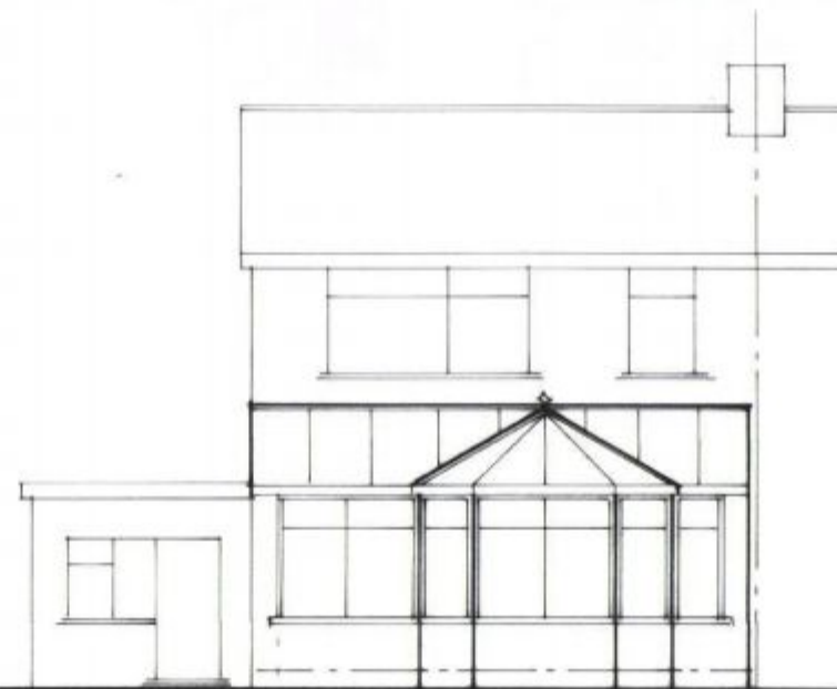
Proposed West/Rear Elevation
