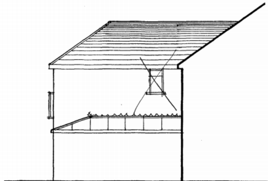
Proposed North/Side Elevation
