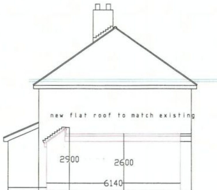
Proposed side elevation(east)
