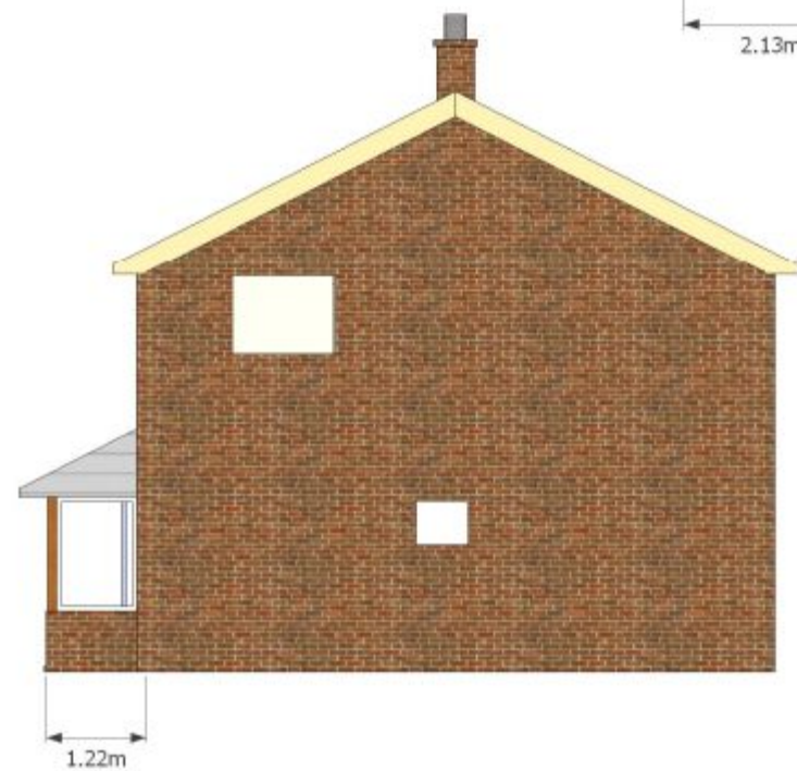
West face elevation
