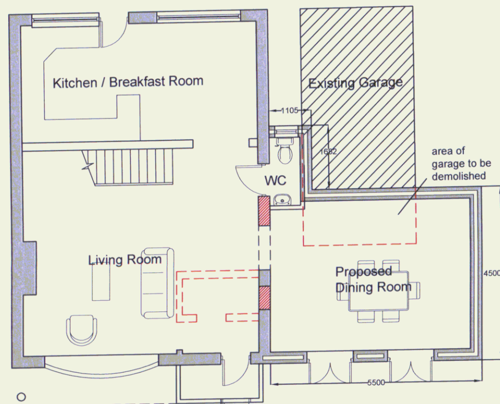
Proposed Ground Floor plan - scale 1:100 @ A3
