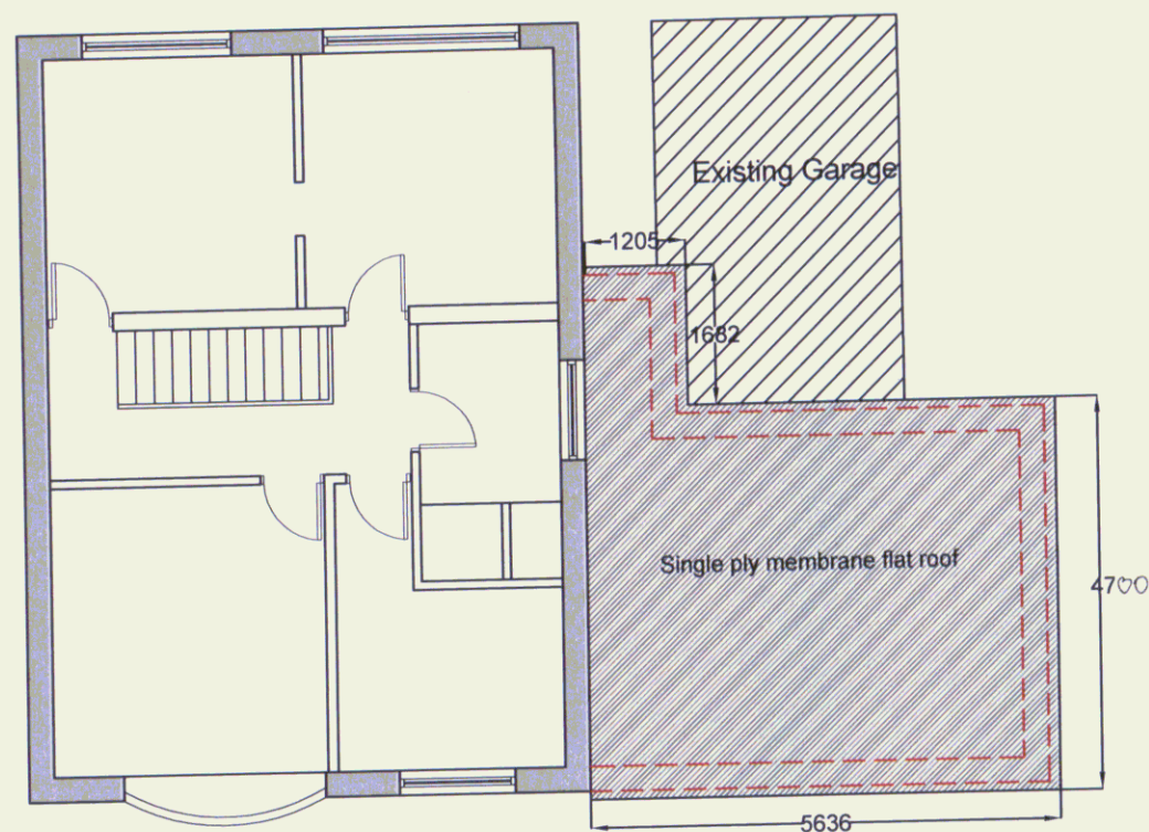
Proposed Roof plan - scale 1:100 @ A3
