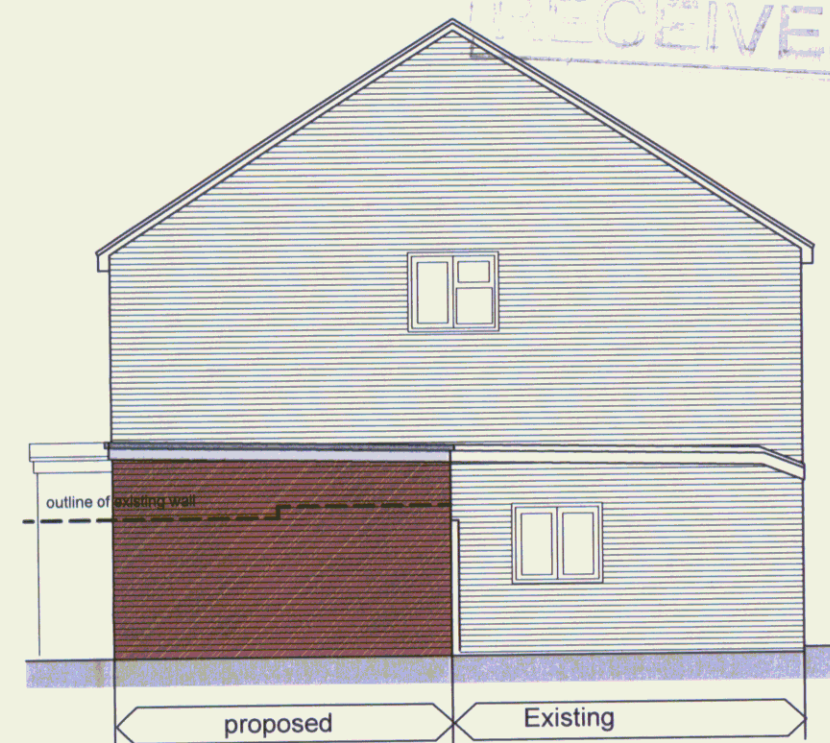
Proposed East elevation - scale 1:100 @A3
