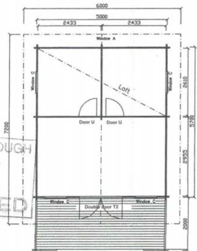
Ground plan
