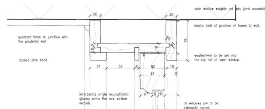
DETAIL 3. scale 1:2
