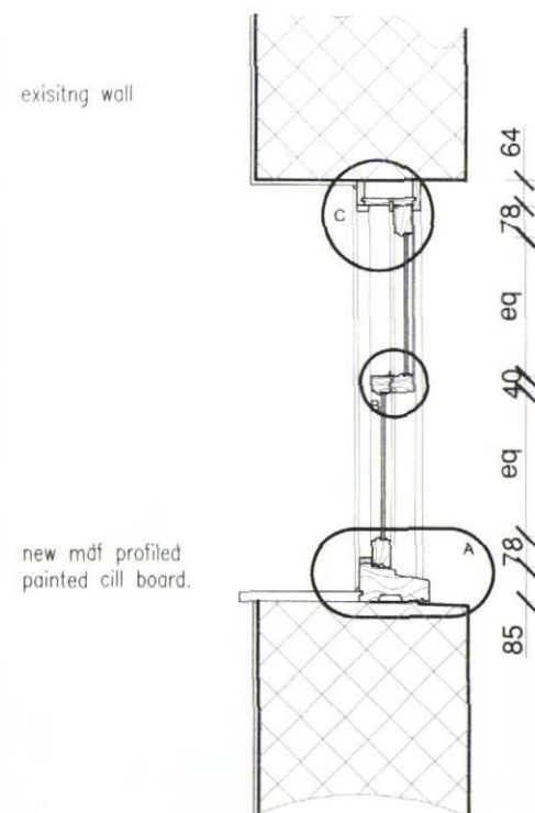
SECTION 3-3.
