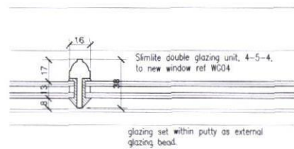
WINDOW WG04 Glazing bar detail. scale 1:2
