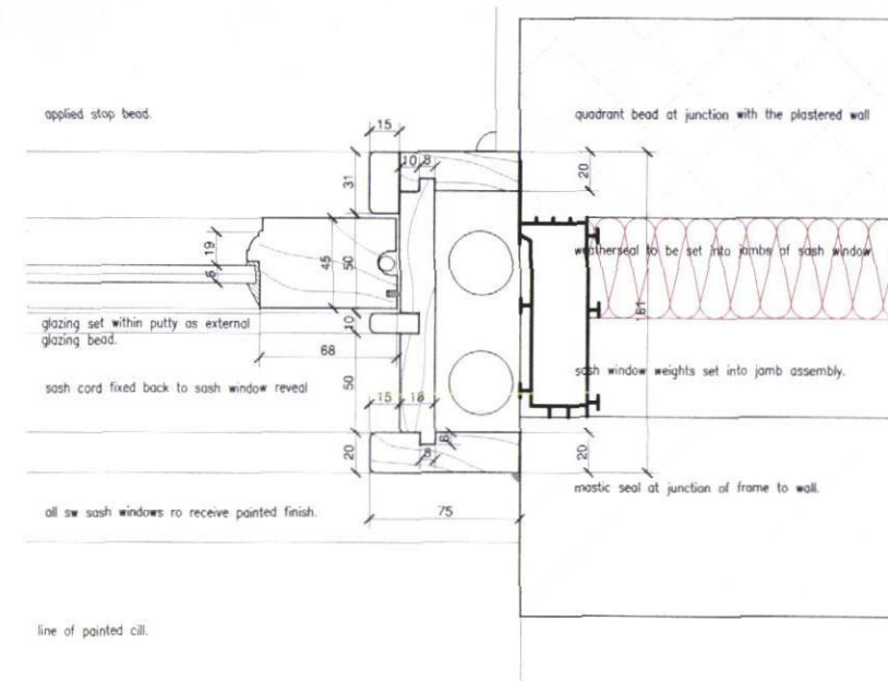
DETAIL 4. scale 1:2
