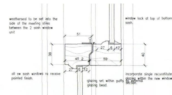
DETAIL 2. scale 1:2
