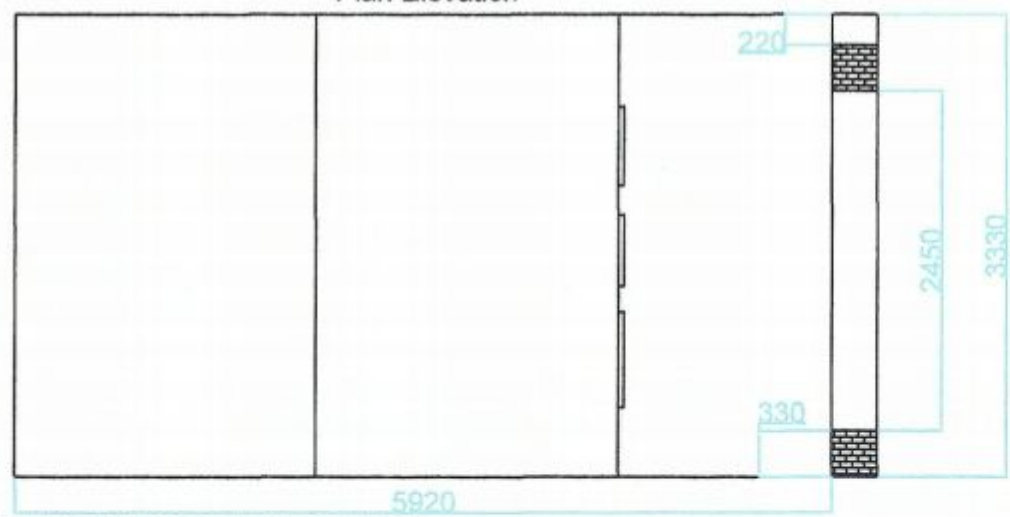
Plan Elevation
