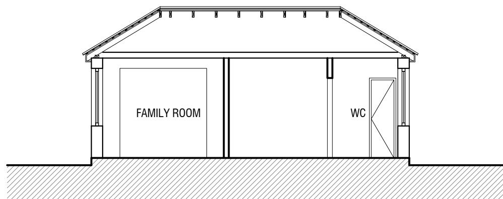
PROPOSED SECTION A-A Scale 1:100
