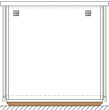
C External View 1:50
