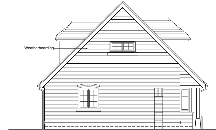
Side Elevation
