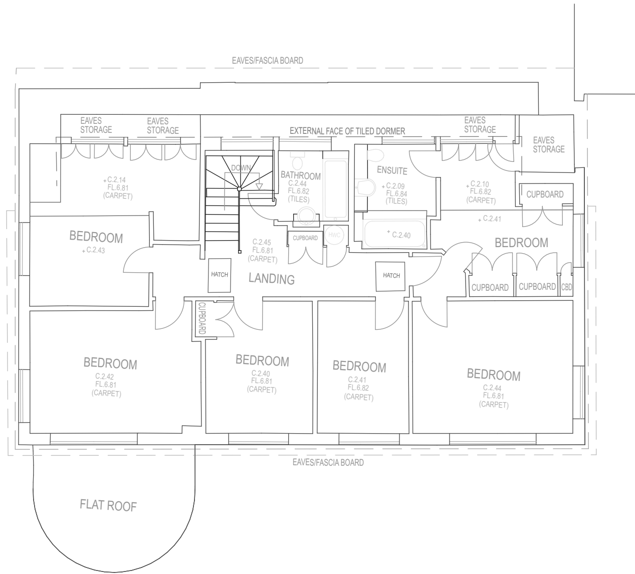
5 - First Floor Existing 1:100
