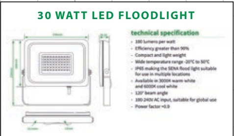
G SEVEN X NEW FLOODLIGHTS SIZE. 0.23m x 168mm. H.A.G. 5m.
