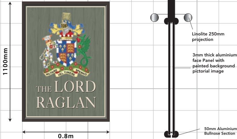
B ONE X NEW DOUBLE SIDED PICTORIAL. NEW LINOLITES SIZE. 0.8m x 1100mm. H.A.G. 3.3m.
