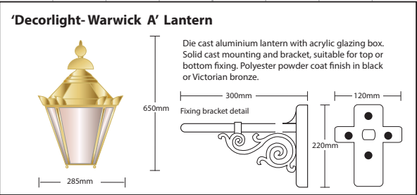
H TWO X NEW LANTERNS SIZE. 0.28m x 650mm. H.A.G. 2.4m.
