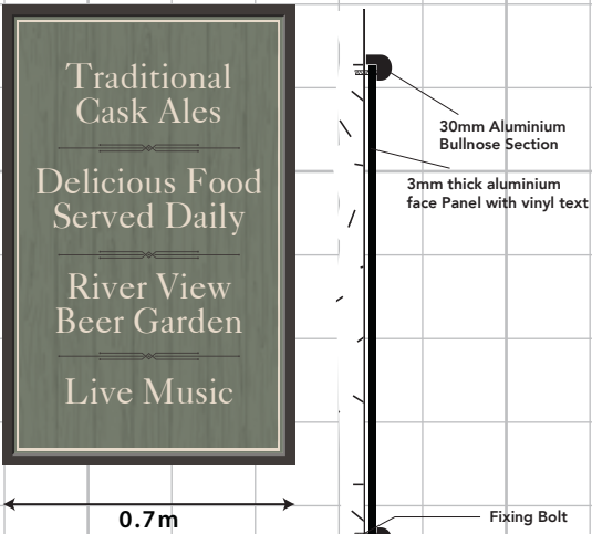
D TWO X NEW AMENITY BOARDS SIZE. 0.7m x 1100mm. H.A.G. 0.8m.
