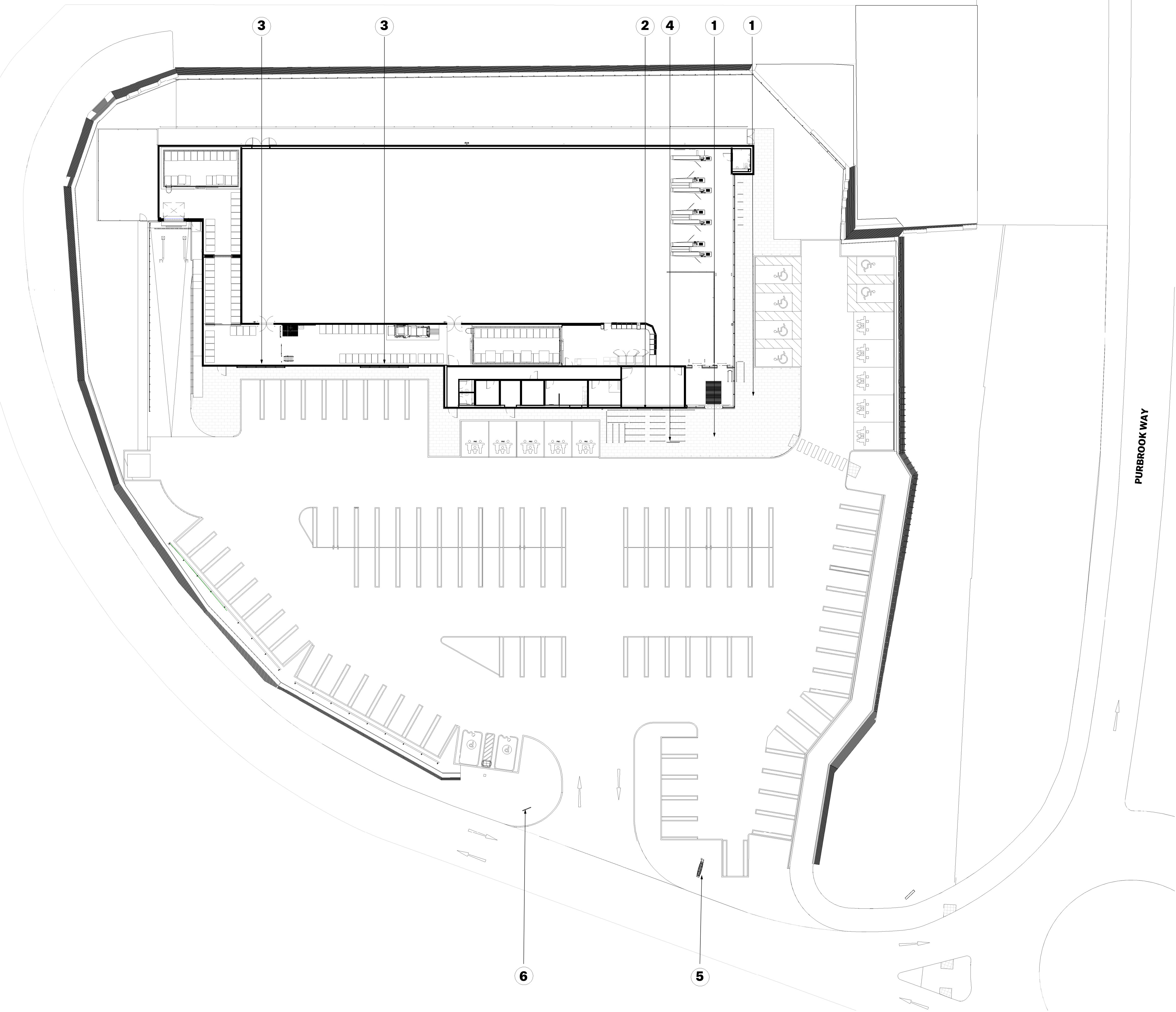
Site Layout Plan - Signage Locations 1: 250
