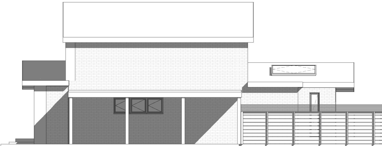
Proposed Elevation-Right side
