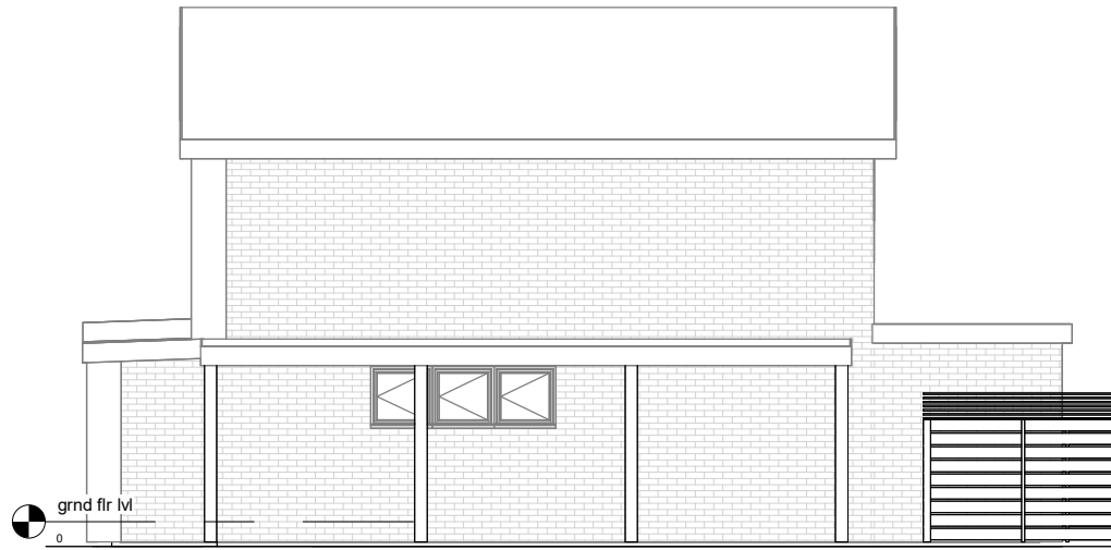
Existing Elevation-Right side
