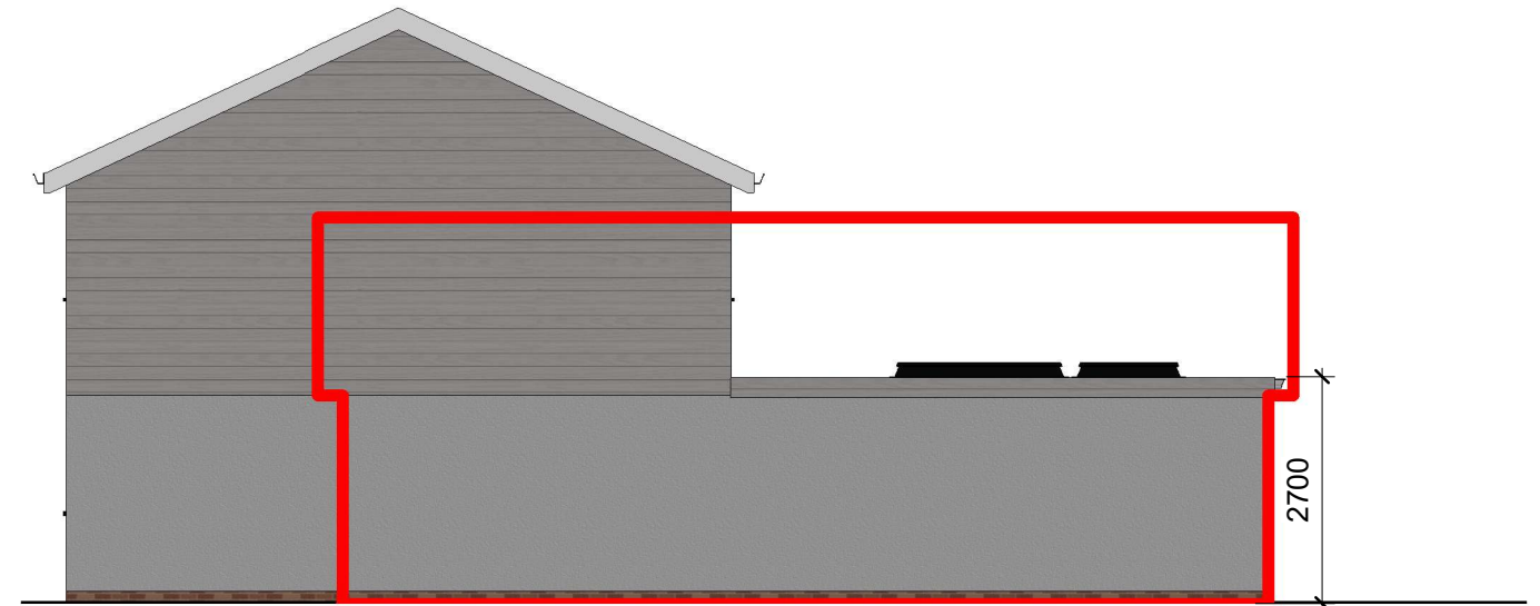
2 North Elevation 1 : 100
