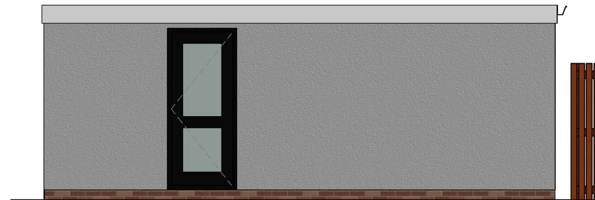
2 Garage Nth Elevation 1 : 50
