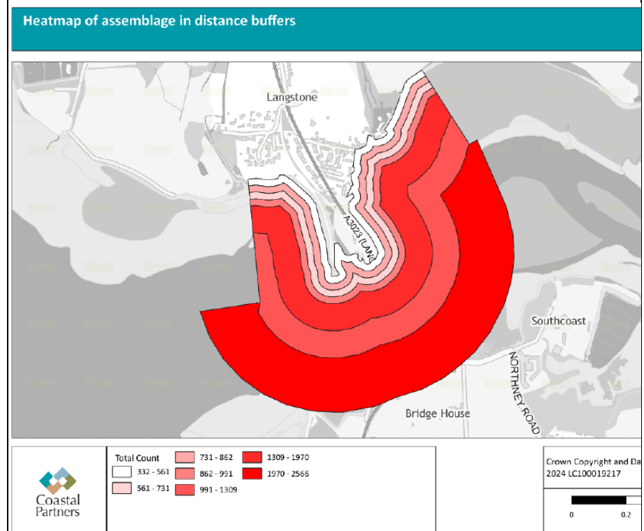
Figure 6. Heatmap of SPA bird assemblage with distance buffers (Coastal Partners, 2025).
