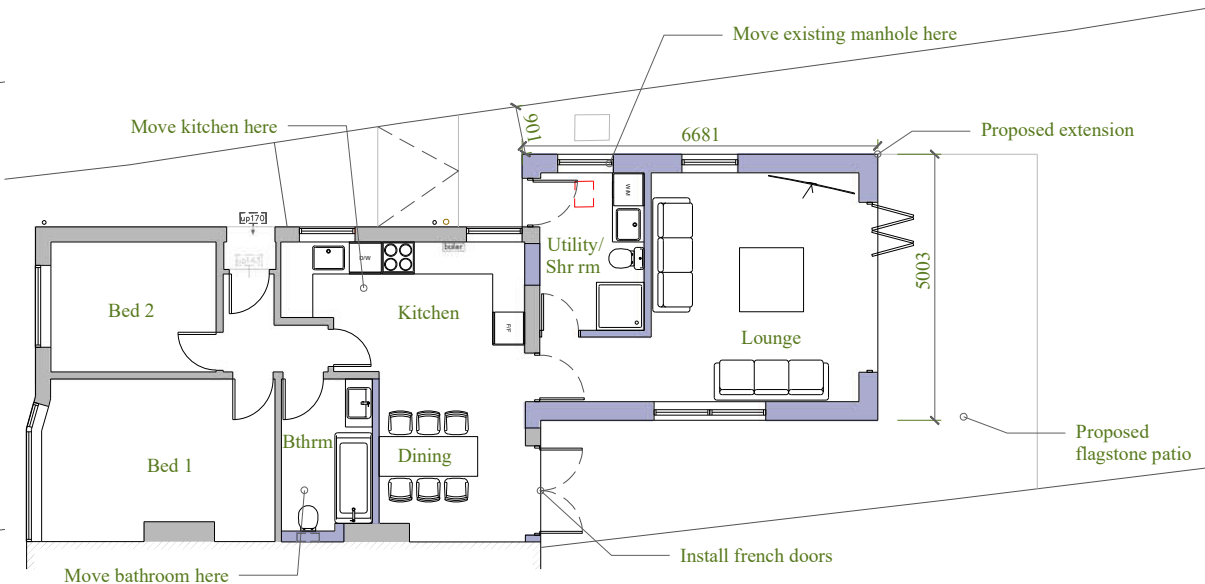
Ground Floor Plan 1:100 PROPOSED
