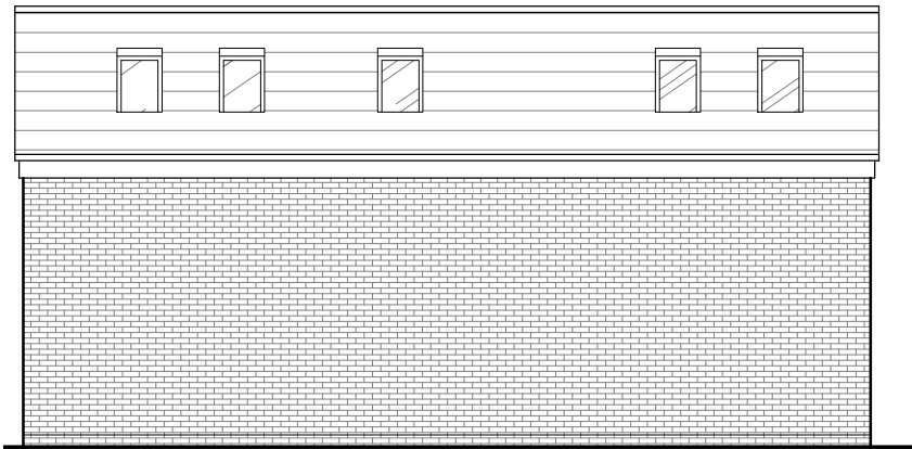
East Elevation 1:100
