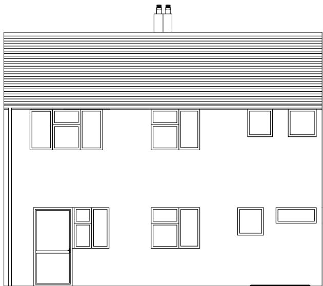
REAR ELEVATION NORTH FACING
