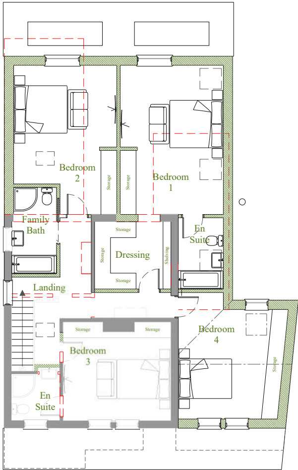
First Floor Plan 1:100 PROPOSED
