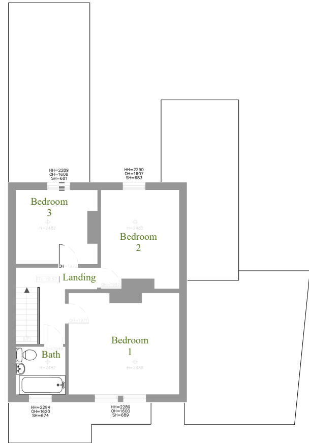
First Floor Plan 1:100 EXISTING
