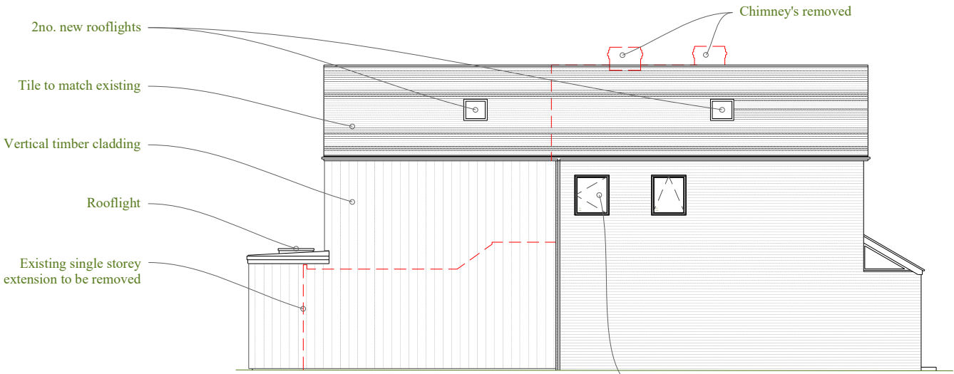
North 1:100 PROPOSED
