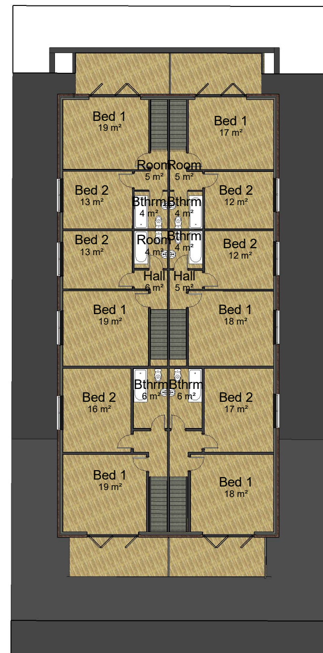
2 X3 Bay TF Plan 1 : 200
