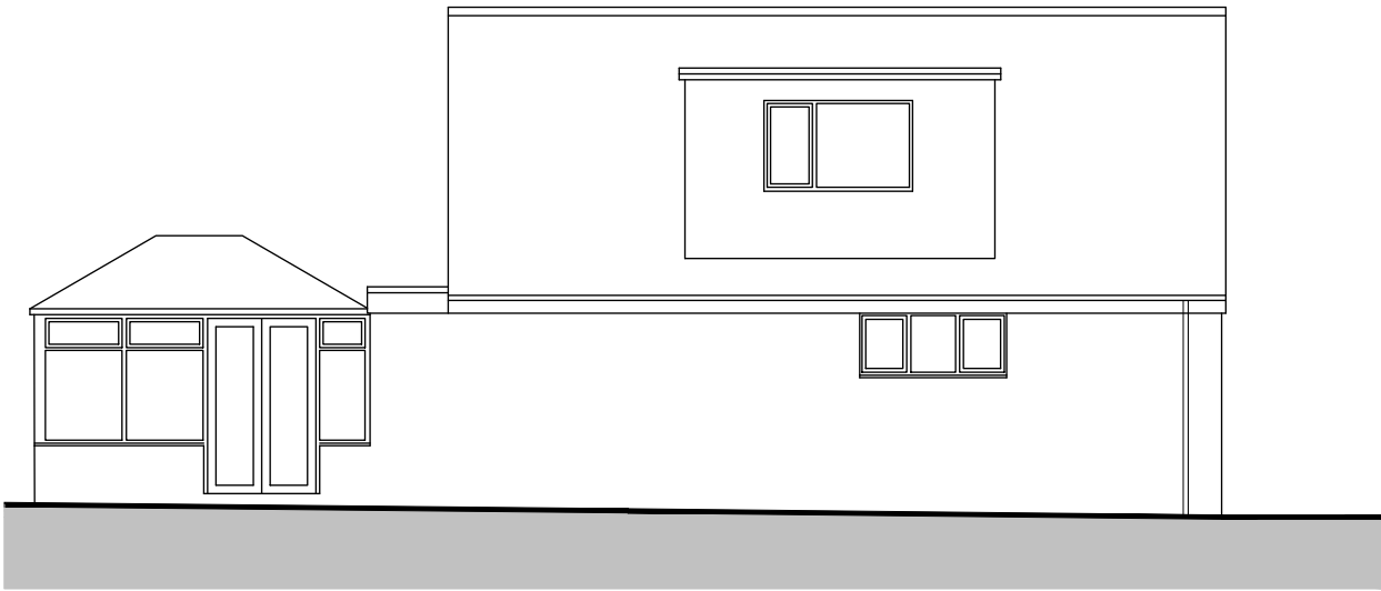
Side Elevation
