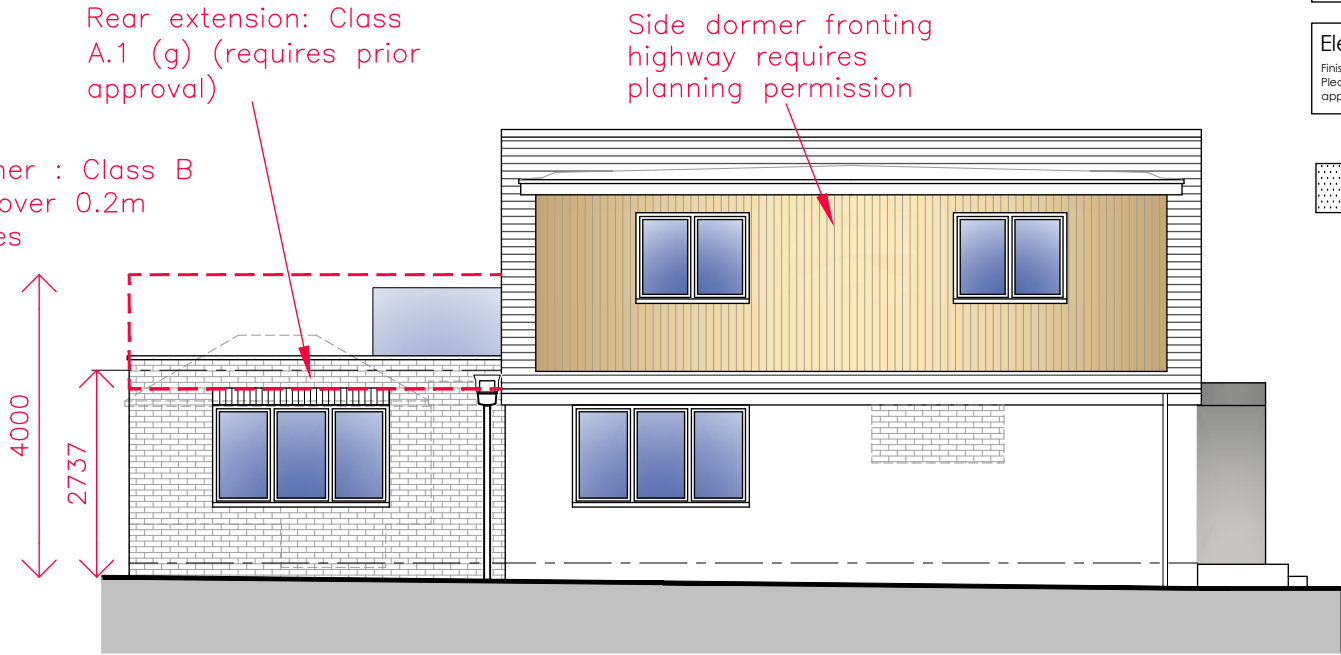
Side Elevation
