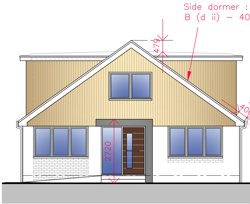
Front Elevation 1:100
